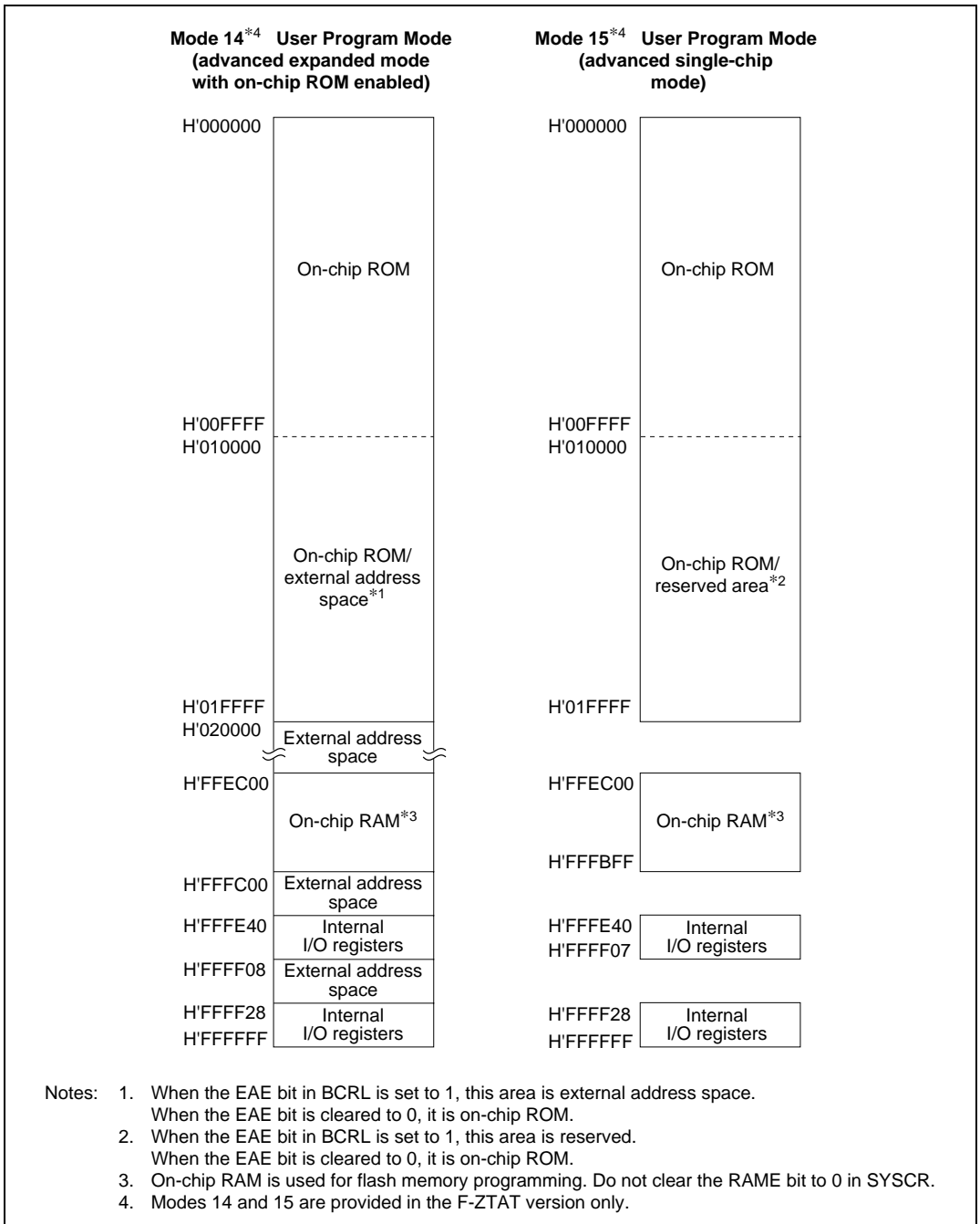
Figure 3.1 Memory Map in Each Operating Mode in the H8S/2345 (cont)
