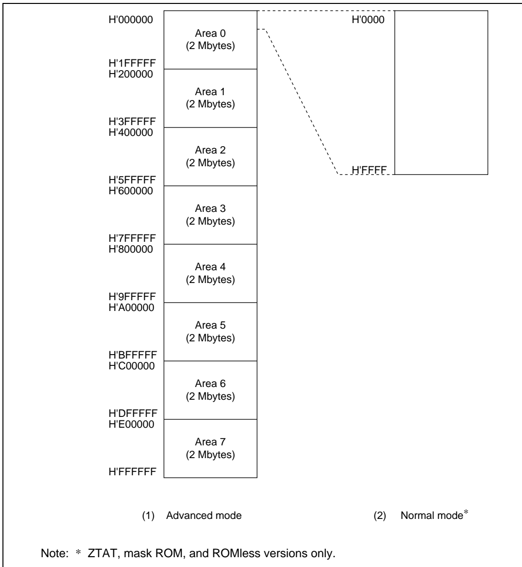
Figure 6.2 Overview of Area Partitioning
