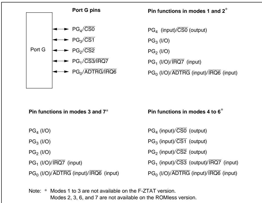
Figure 8.24 Port G Pin Functions
