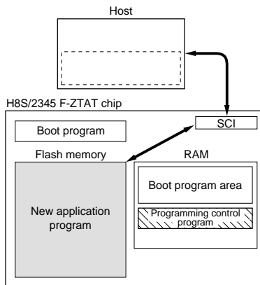
Figure 17.9 Boot Mode
