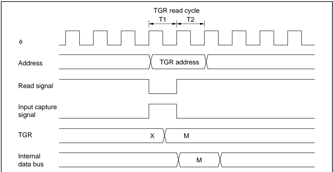
Figure 9.53 Contention between TGR Read and Input Capture
