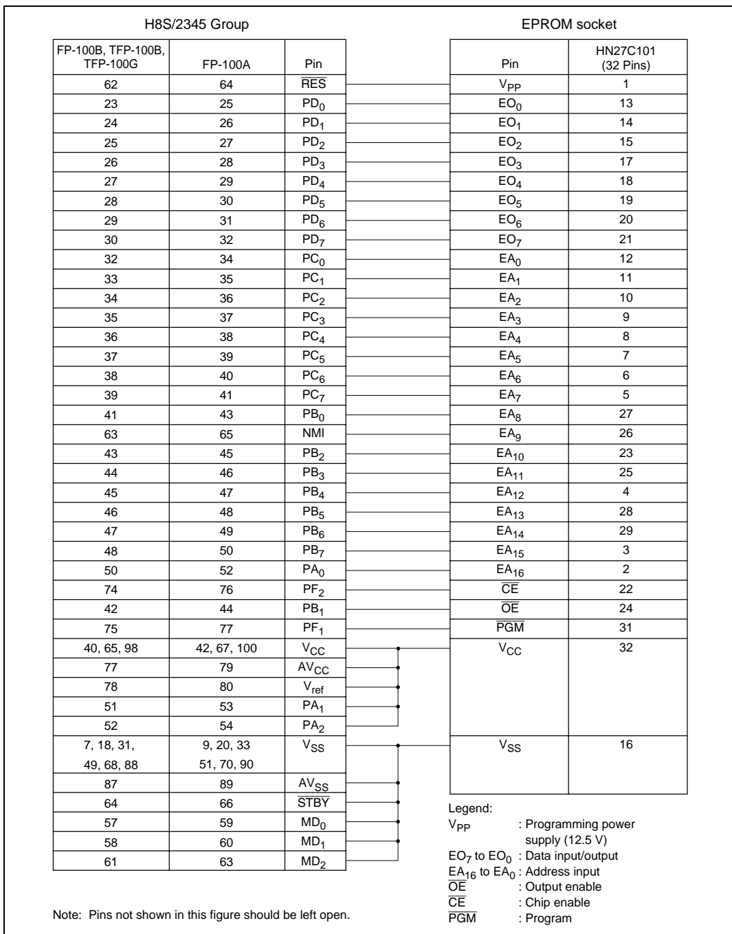
Figure 17.2 Wiring of 100-Pin/32-Pin Socket Adapter
