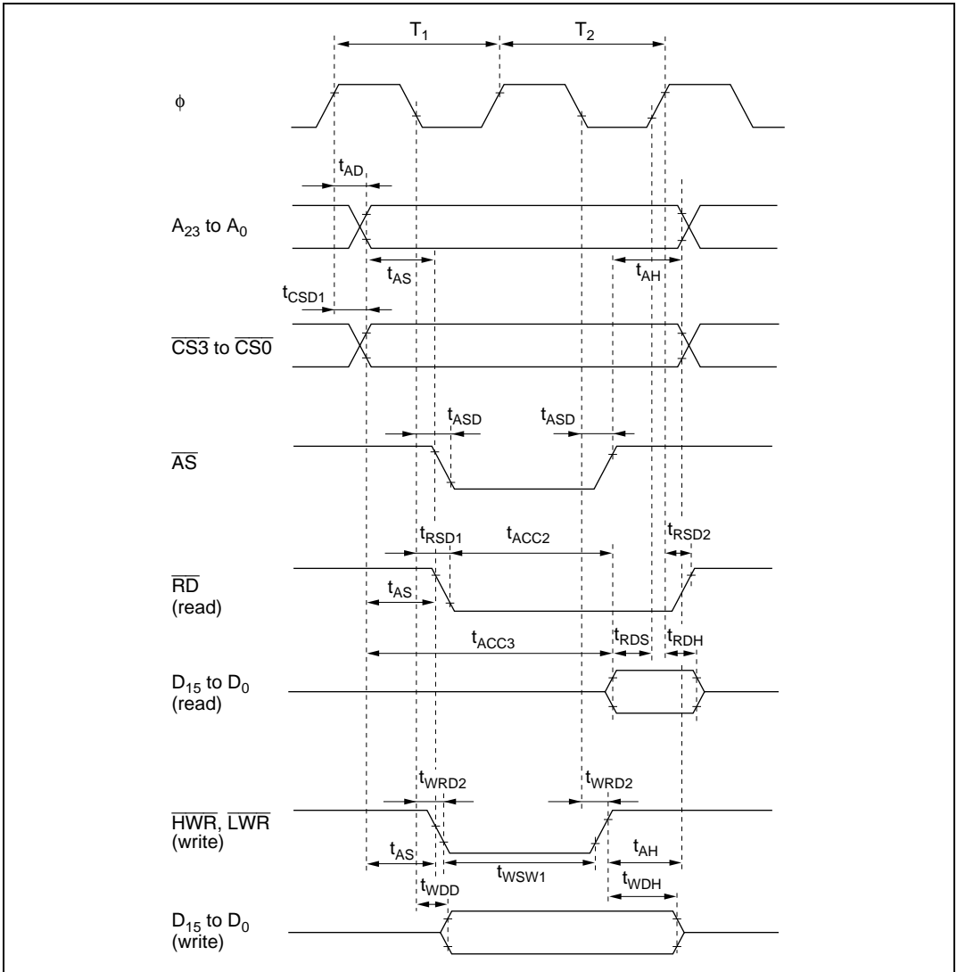
Figure 20.11 Basic Bus Timing (Two-State Access)
