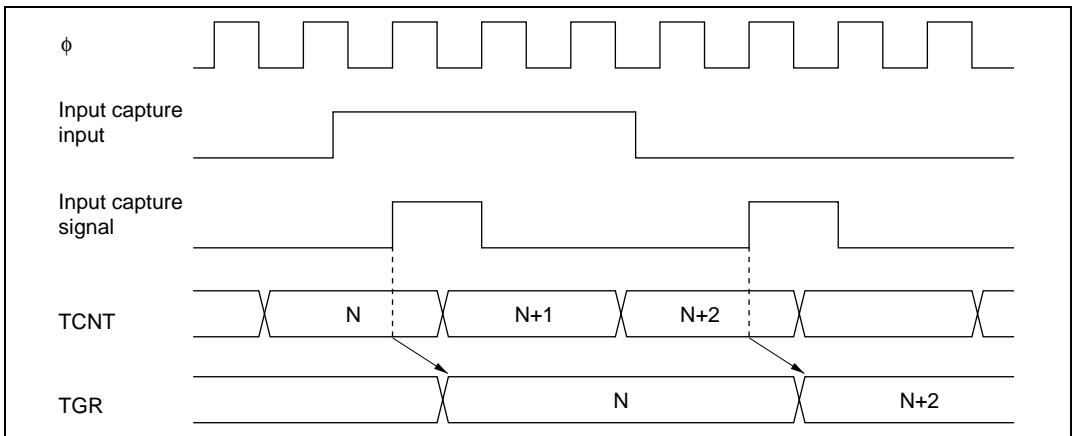
Figure 9.37 Input Capture Input Signal Timing
