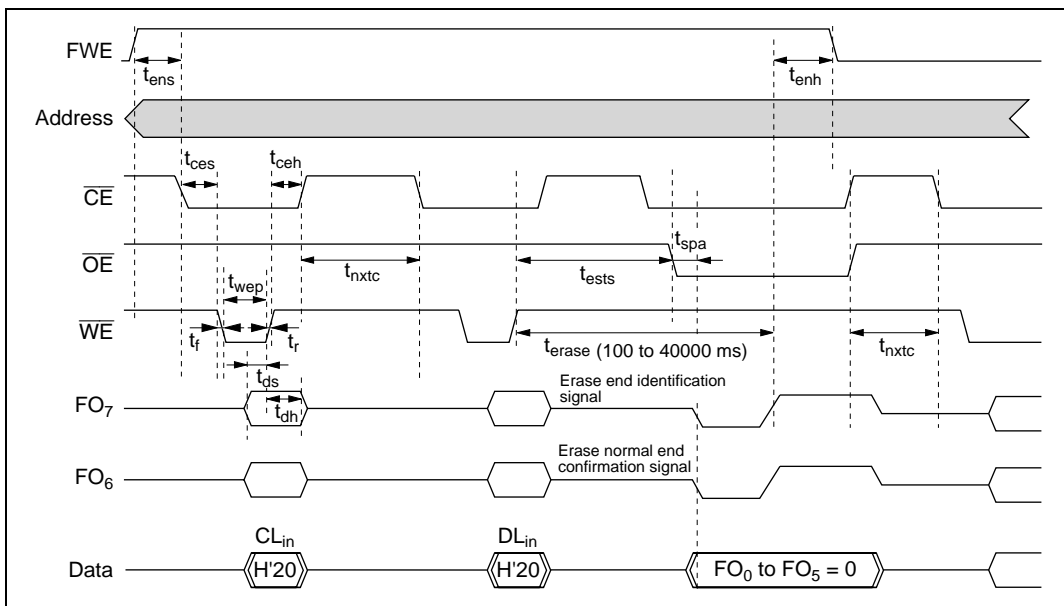
Figure 17.32 Auto-Erase Mode Timing Waveforms
