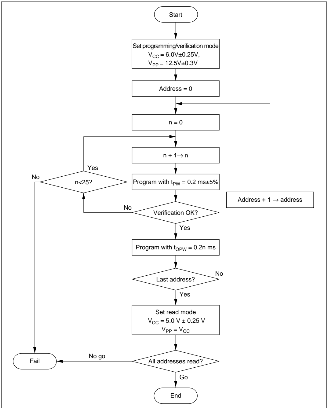
Figure 17.4 High-Speed Programming Flowchart
