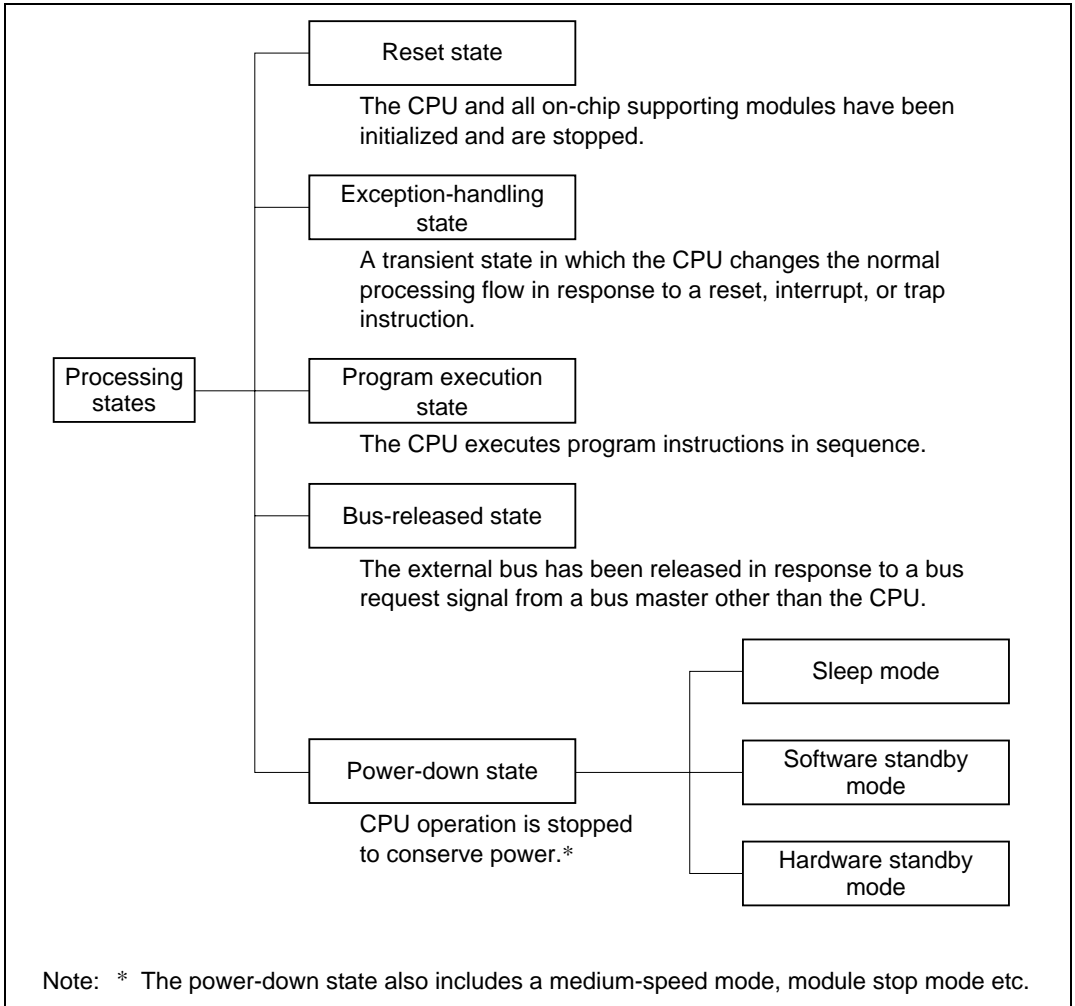
Figure 2.14 Processing States
