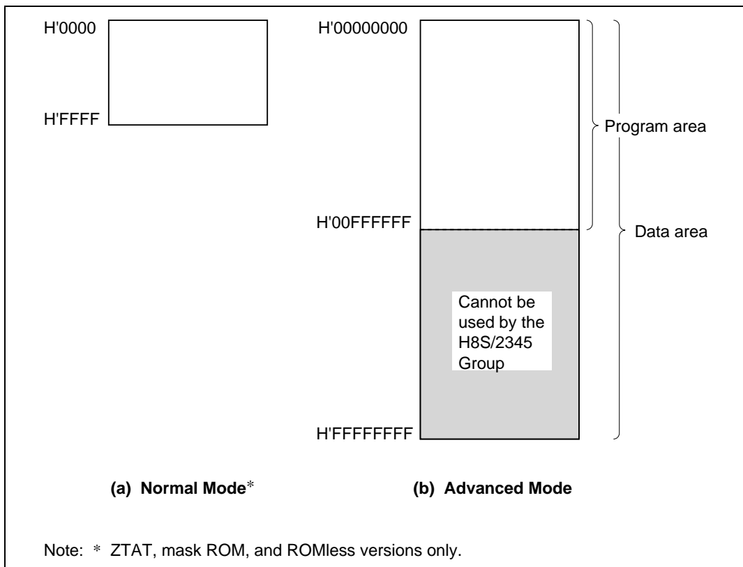
Figure 2.6 Memory Map
