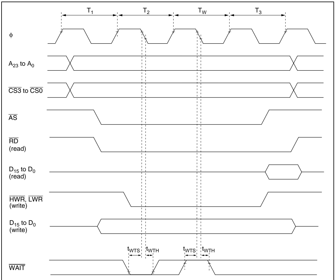
Figure 20.13 Basic Bus Timing (Three-State Access with One Wait State)
