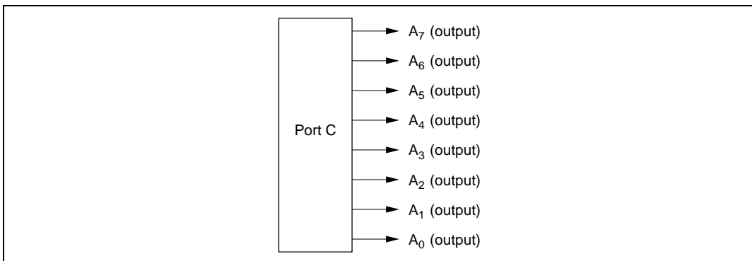
Figure 8.14 Port C Pin Functions (Modes 1, 4, and 5)*
