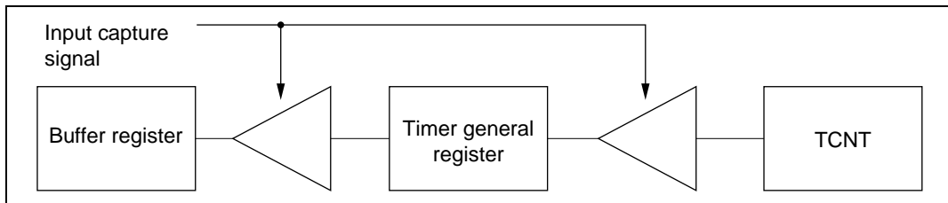
Figure 9.17 Input Capture Buffer Operation
