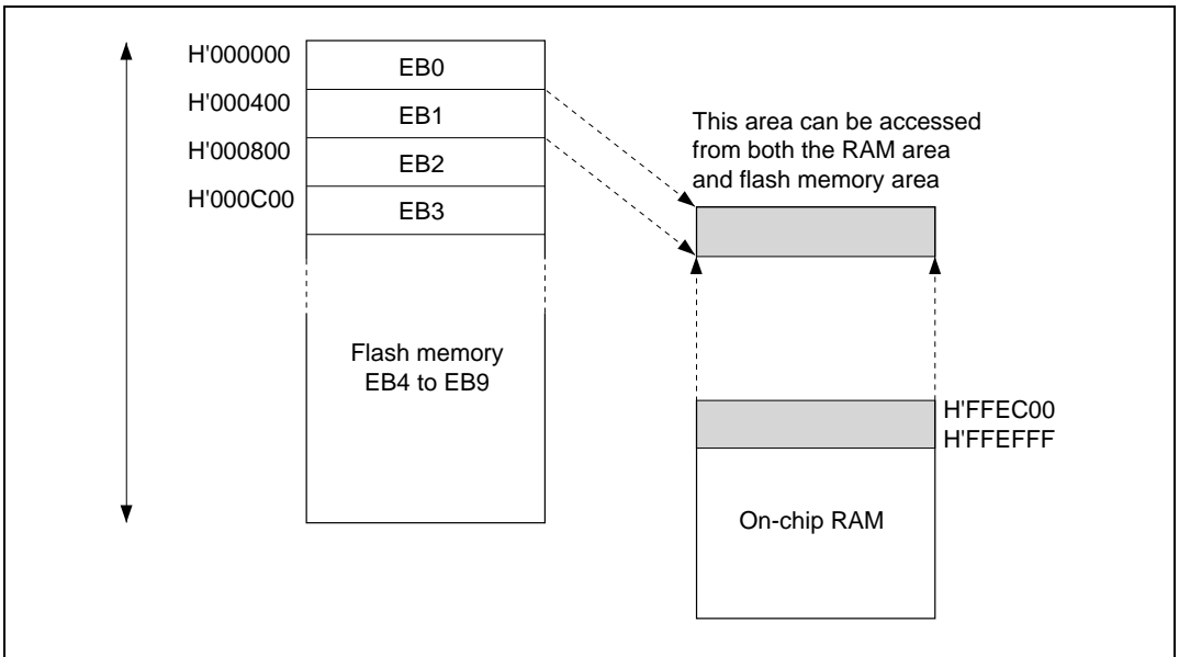
Figure 17.25 Example of RAM Overlap Operation
