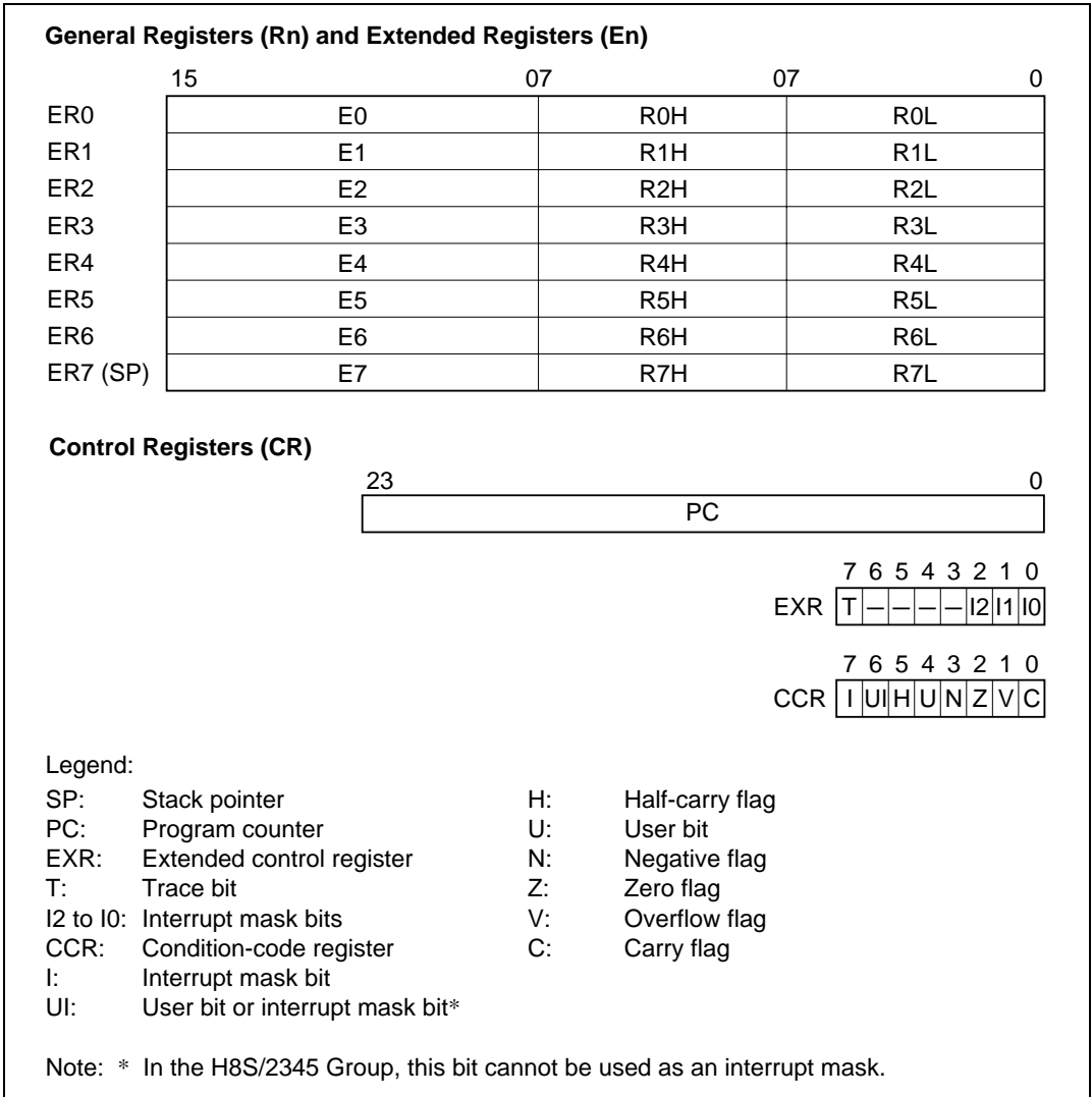
Figure 2.7 CPU Registers
