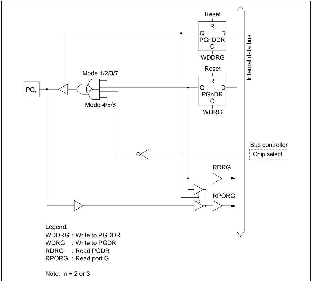
Figure C.11 (c) Port G Block Diagram (Pins PG_2 and PG_3 )
