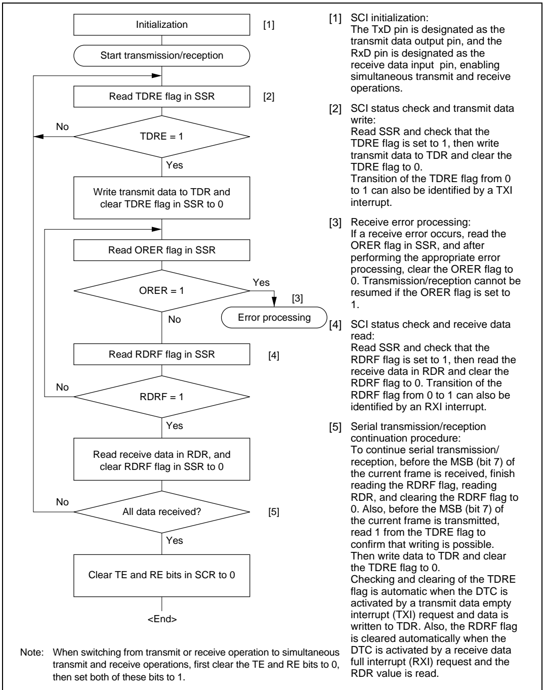
Figure 12.20 Sample Flowchart of Simultaneous Serial Transmit and Receive Operations
