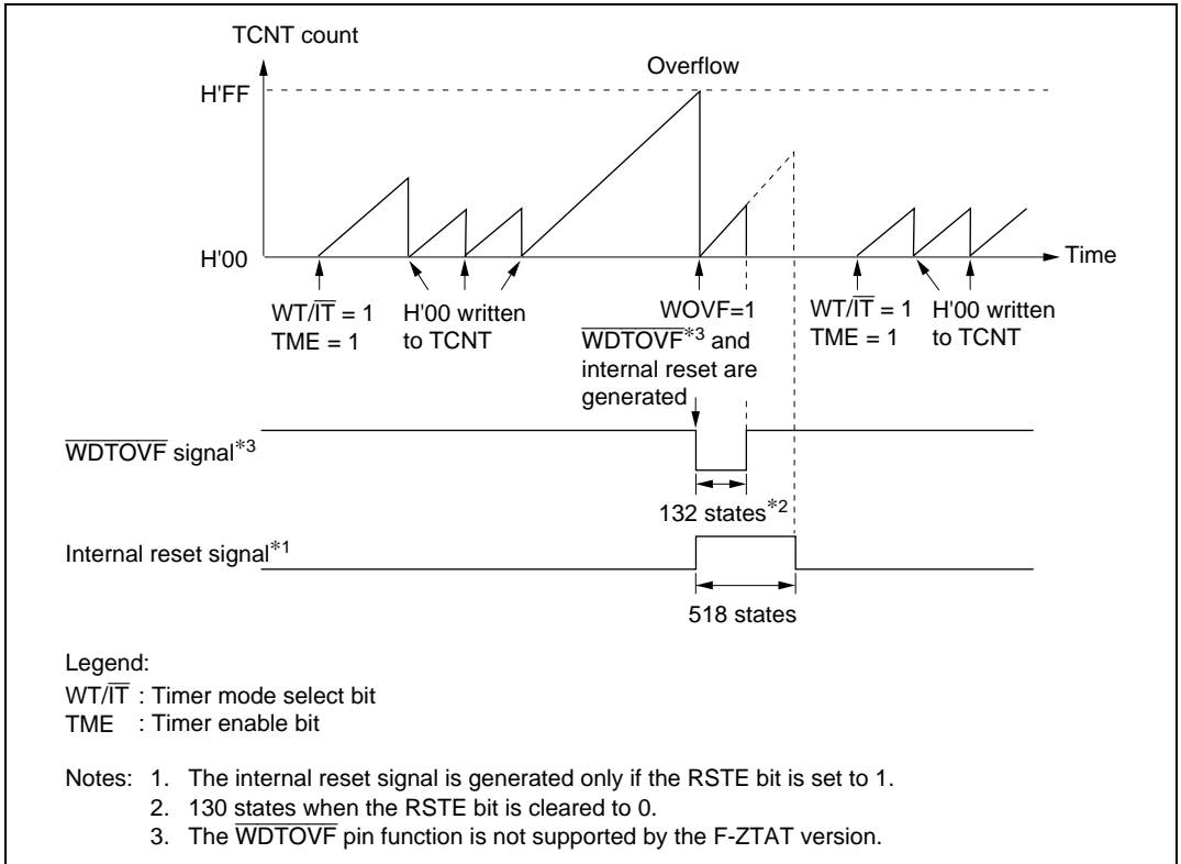
Figure 11.4 Watchdog Timer Operation
